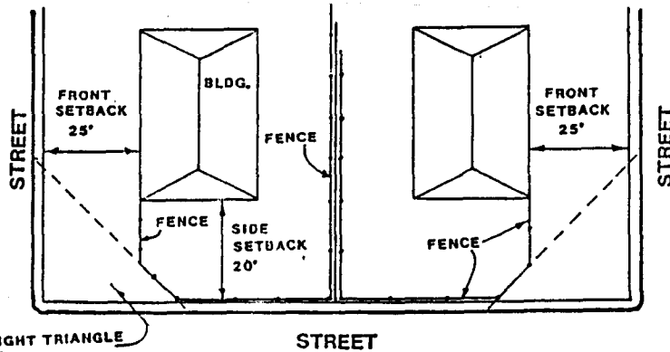
SIGHT TRIANGLE AS DEFINED BY CITY CODE
